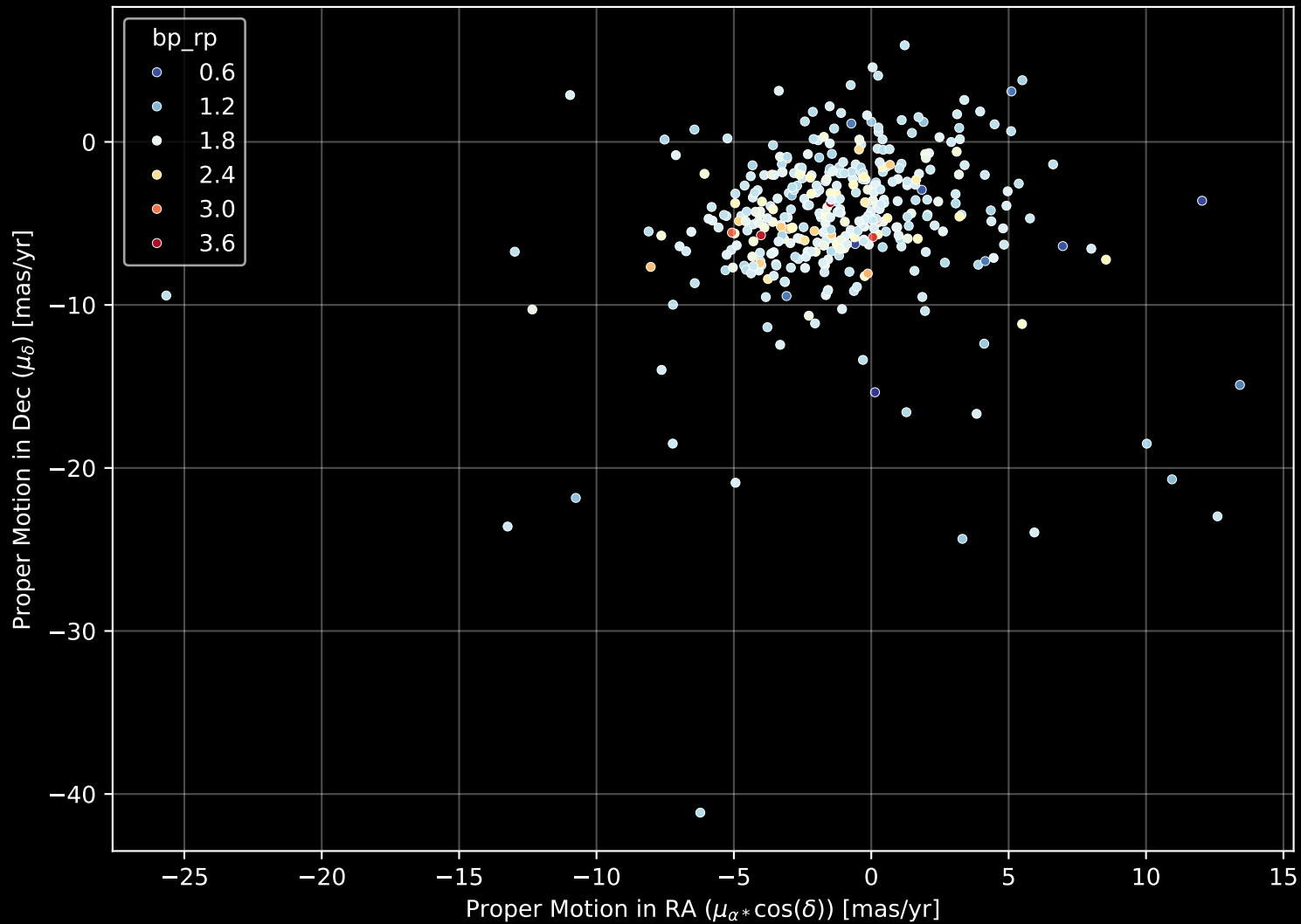
APOGEE DR17 Field: [010-12] Proper Motion Diagram (n= 379)
