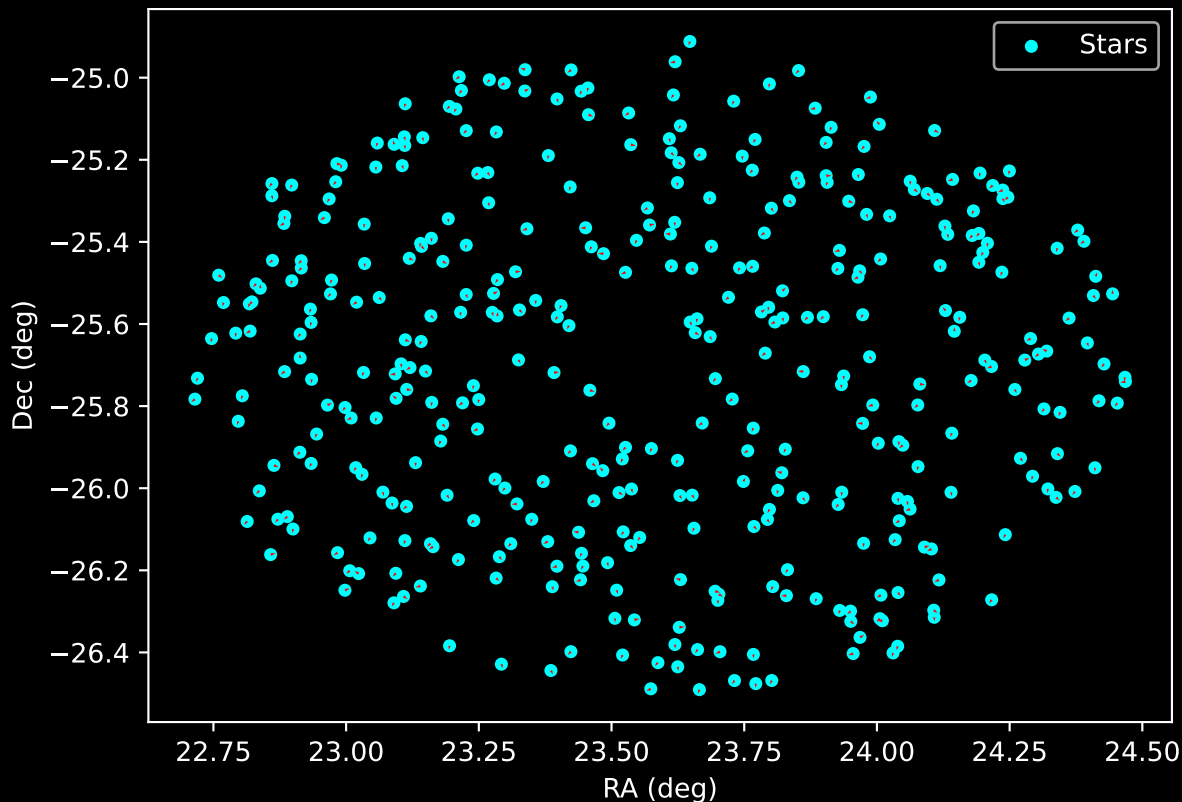
APOGEE DR17 Field: [010-12] Proper Motion Vectors for Gaia Star Field (n= 379)
