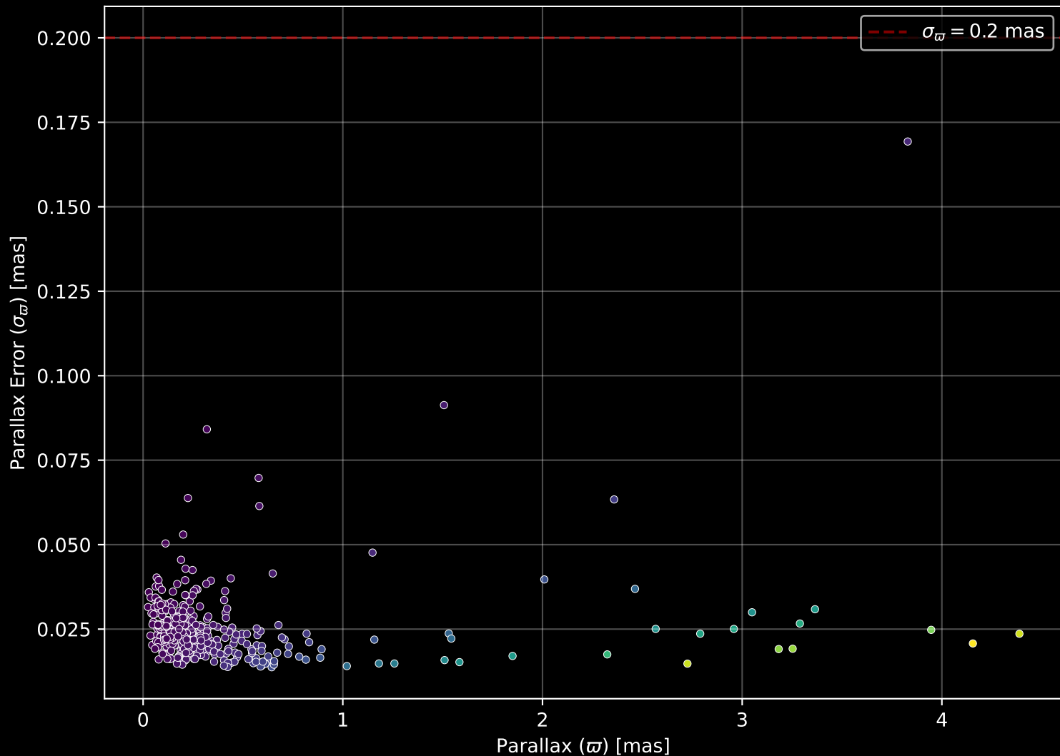
APOGEE DR17 Field: [010-12] Parallax Quality (n= 379)
