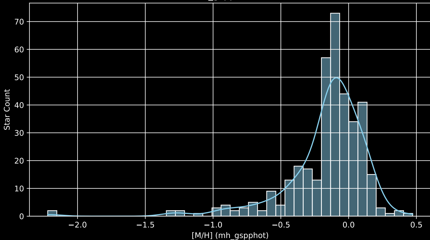
APOGEE DR17 Field: [010-12 [M/H] (mh_gspphot) (n= 371)
