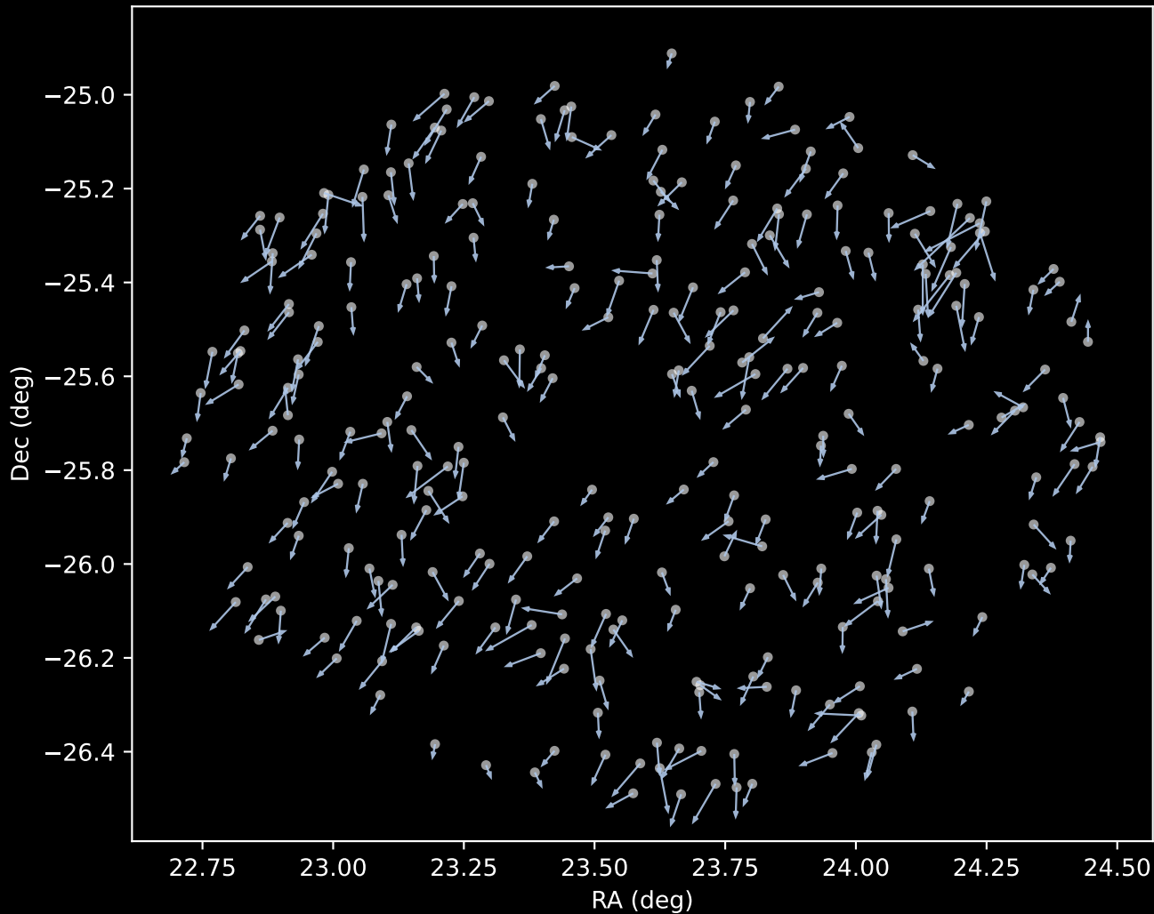
APOGEE DR17 Cluster 1 Proper Motion Vectors (n=290)
