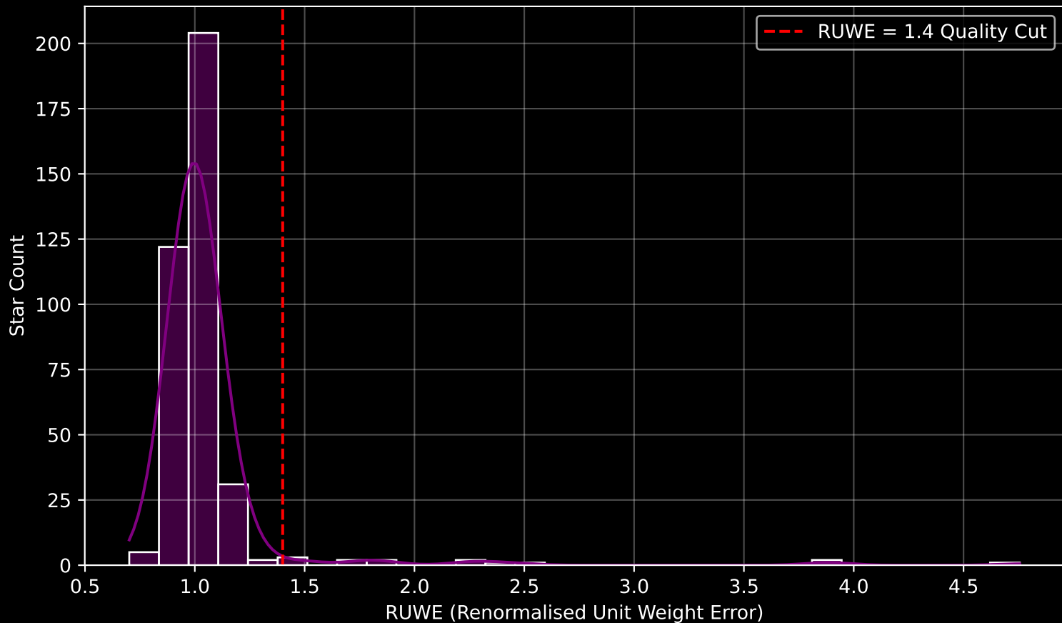
GAPOGEE DR17 Field [010-12] RUWE Distribution (n= 378)
